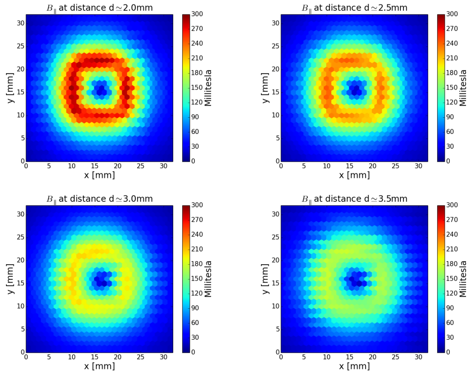
Figure A.1.: Horizontal magnetic field at various distances above the magnet 5.
