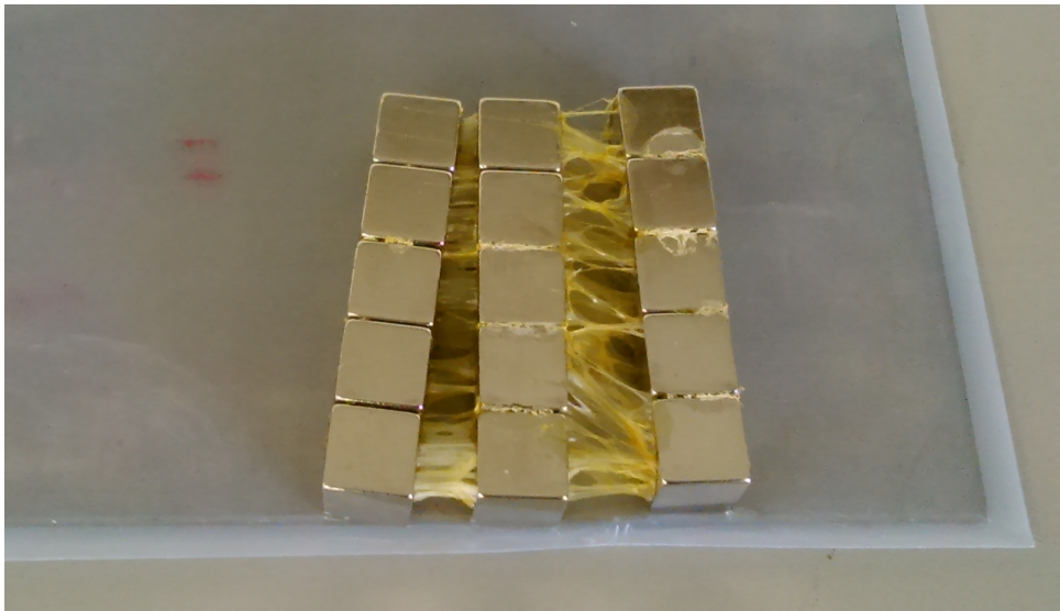
Figure 5.23.: The result of the first failed attempt. These three stripes could be pushed together, but it was not possible to push them further towards the remaining two stripes. Although still attracted by the small iron plate, they moved a little bit away from each other due to their repellent forces. This is indicated by the glue between them: to end up in this state, the inner surfaces must have been so close that the glue drops applied to them were in contact with each other. Apparently, the glue was insufficiently strong to hold the magnets together and was elongated instead.
