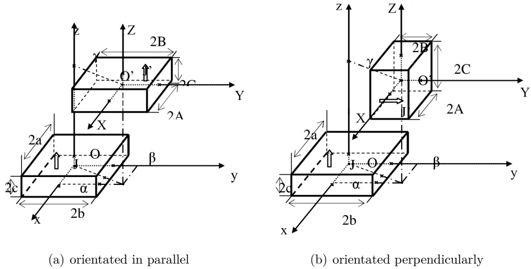
Figure 3.7.: Orientation of the two magnets relative to each other. This sketch is the basis of the force calculations. In both cases, a, b, c, A, B, C are half the edge lengths of the magnets and \alpha, \beta, \gamma are the distances of the centres with regard to the x -, y -, z -axis respectively. In the perpendicular case, if both magnetizations have a positive leading sign, the first one points towards the positive z -direction and the second one points towards the positive y -direction. From [80].
