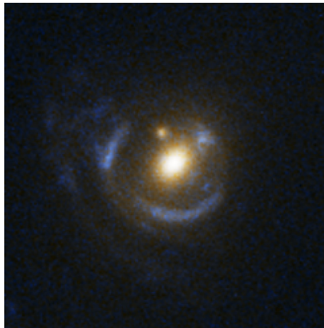
Figure 2.2.: Example of the gravitational lensing. Due to this effect the background light source appears as a part of a ring. Such a ring is also called “Einstein ring”. From [15].
