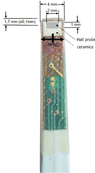
Figure 5.3.: A sketch of the Hall probe used for the magnetic field measurements. The tip of the probe contains the active area, which is surrounded by ceramics. This area has the size 1\text{ mm} \times 2\text{ mm} and its middle is 1.7\text{ mm} inside the tip.
