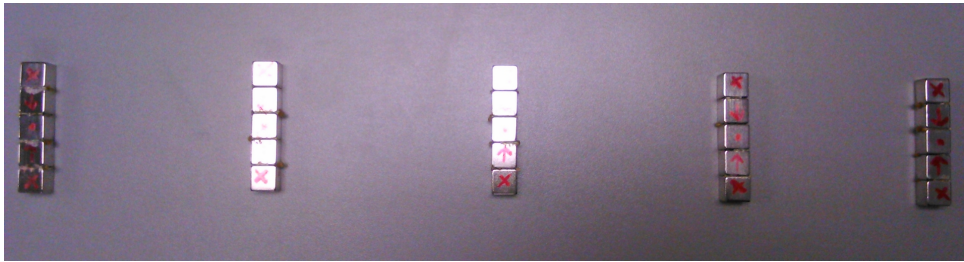
Figure 5.19.: The five 5x1 Halbach stripes constructed to be the components of the 5x5 Halbach array. The symbols on the upper surfaces are analogue to the ones in figure 5.10. The distance between them is nearly the minimal distance without them reacting to each other.
