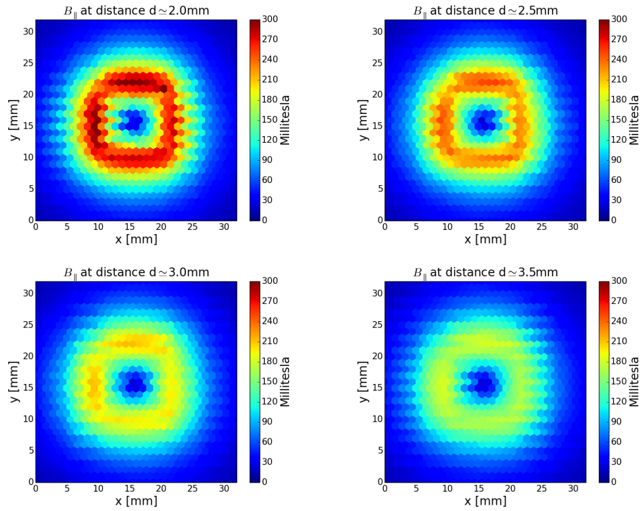
Figure A.9.: Horizontal magnetic field at various distances above the magnet 13.
