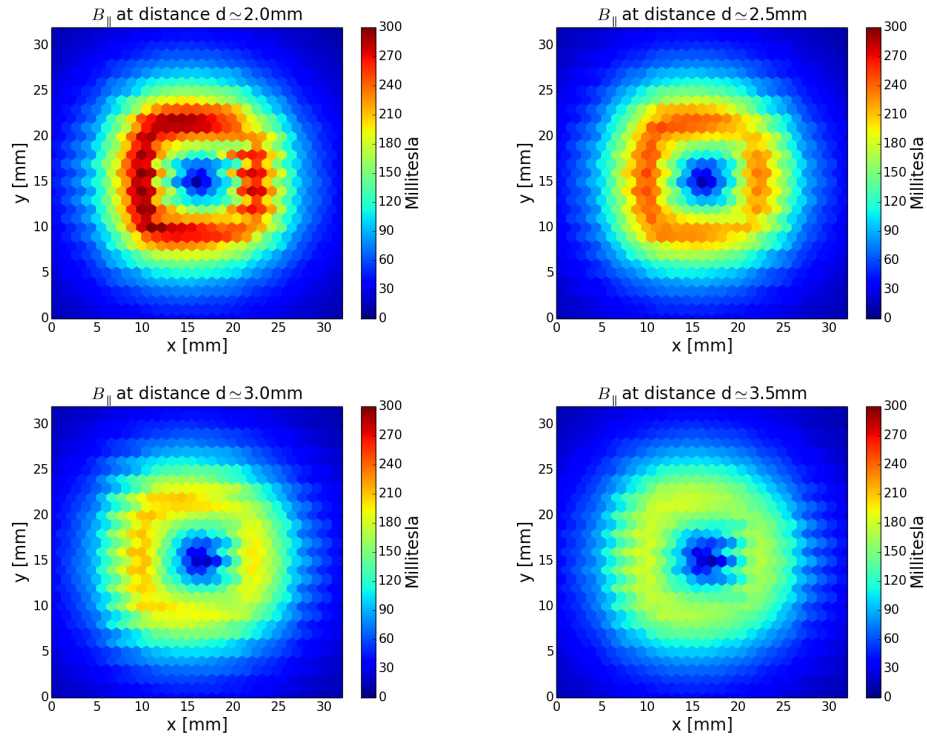
Figure A.4.: Horizontal magnetic field at various distances above the magnet 8.
