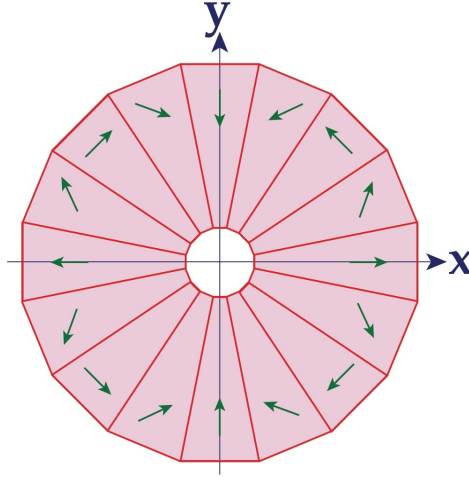
Figure 3.5.: A scheme of the cross section of the quadrupole built by Halbach. With its trapezoidal components and the self-contained structure it differs strongly from Mallinson's tape. Nevertheless, the main principle, i.e. the rotation of consecutive magnetization vectors by a fixed degree, is equal in both cases. From [8].
