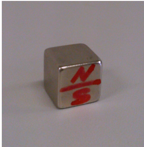
Figure 5.1.: A single cubic magnet used for the preliminary measurements for BRASS. The magnetization direction lies parallel to the centre line between the upper and the lower faces in this picture.
