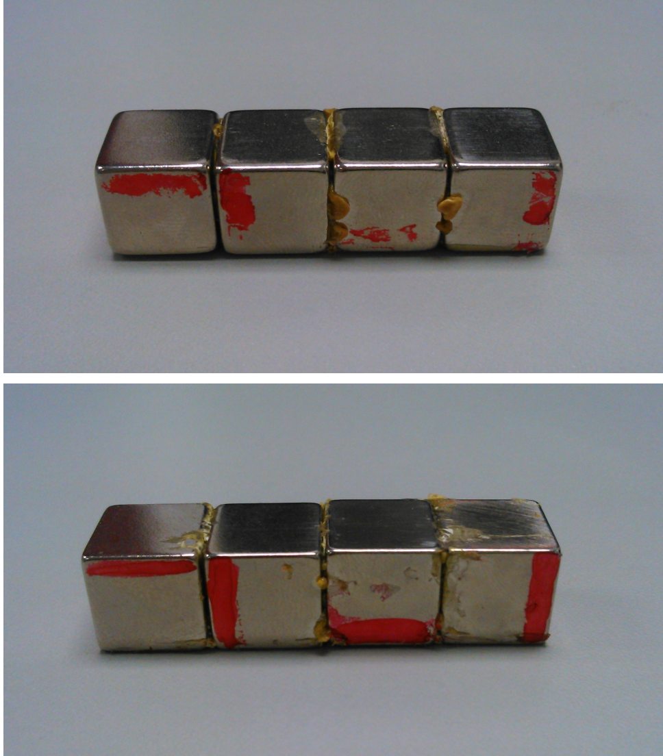
Figure 5.16.: The 2 constructed 1D Halbach units. The red bars indicate the south poles of the magnets. It is clearly visible that there is some space between the individual magnets due to the glue. The unit is therefore slightly wider than the sum of the 4 magnets. In the middle of the lower unit it is also visible that the arrangement is not perfectly planar. This also applies to the upper unit, though it is harder to see in this image.
