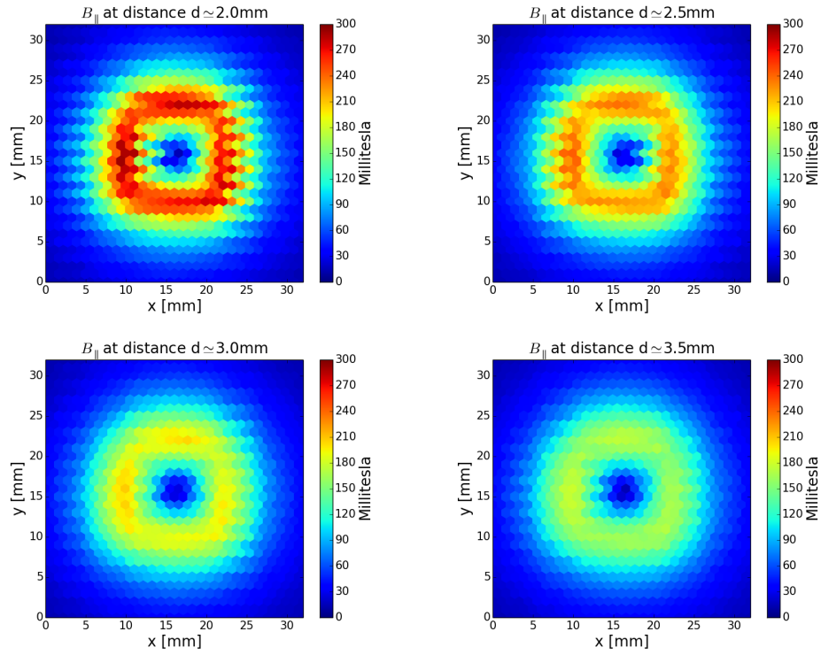
Figure A.14.: Horizontal magnetic field at various distances above the magnet 18.
