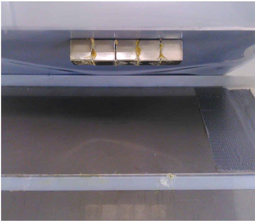
Figure 5.12.: The glued magnets from figure 5.11(b) after detaching them after the glue hardened. Since the magnetic field is stronger on the upper side, the array sticks to the upper plate. This plate is smaller and it is therefore easier to release the array afterwards from this one than from the bigger lower plate.
