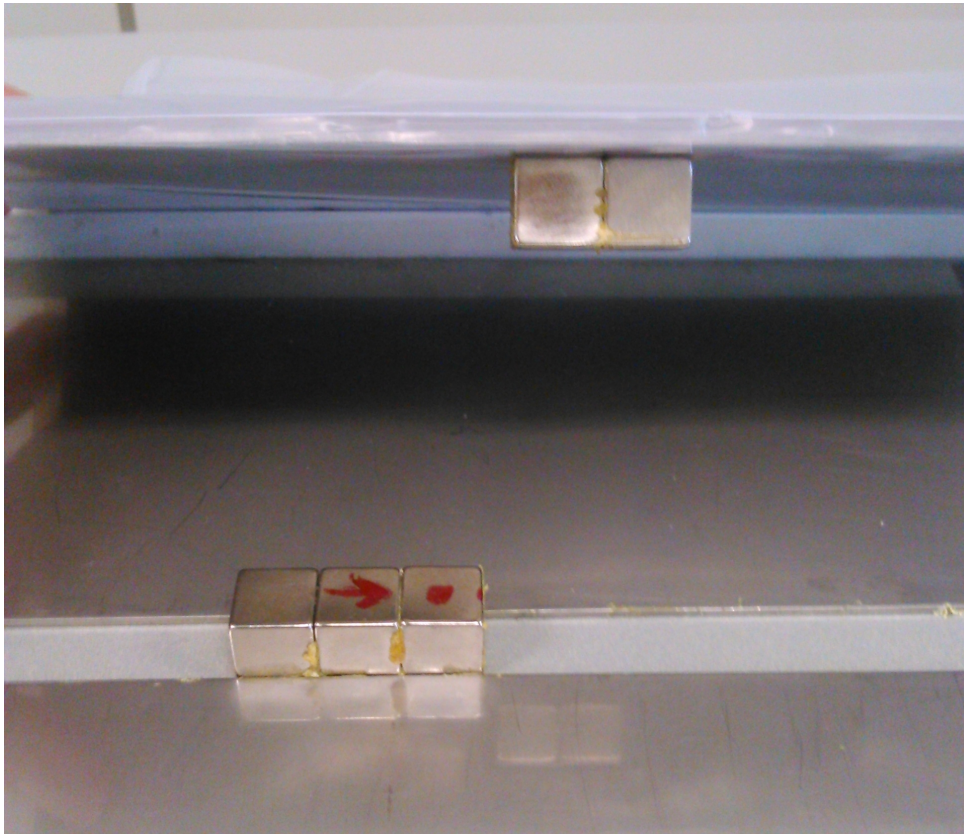
Figure 5.14.: A 5x1 array damaged while being detached from the lower plate. As a result of glue seeping between the three magnets on the left and the lower plate, their attraction was stronger than the adhesive attraction between the three magnets on the left and the two magnets on the right. Hence, the attempt to detach the array resulted in the breaking of the array.
