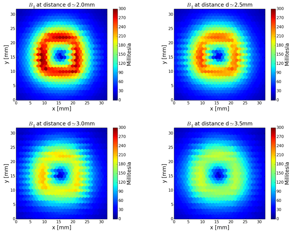
Figure A.7.: Horizontal magnetic field at various distances above the magnet 11.
