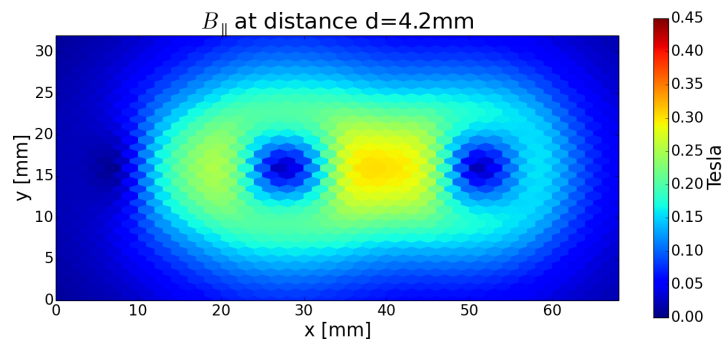
(c) Computation at 4.2 mm above the unit
