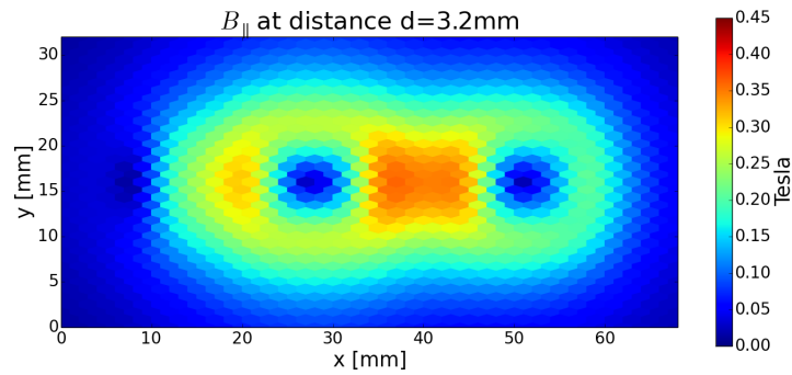
(c) Computation at 3.2 mm above the unit
