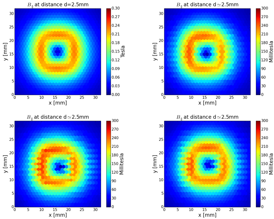
Figure 5.5.: Computed (top left) and measured horizontal magnetic field of single magnets at a distance d = 2.5 mm.
