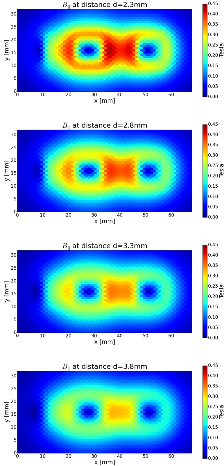
Figure 4.2.: The results of the magnetic field computations of a 1D Halbach unit. The plots show the field at distances d = 2.3\text{ mm}, 2.8\text{ mm}, 3.3\text{ mm}, 3.8\text{ mm} . The array is located such that 10 \leq x \leq 58 and 10 \leq y \leq 22 .
