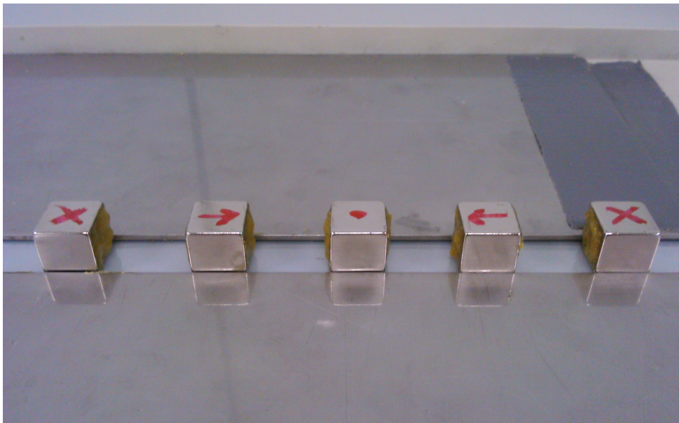
Figure 5.10.: Magnets placed inside the rail with glue put on the inner faces. The marks on the upper faces indicate the direction of magnetization; the arrows point towards the south pole which is indicated by the dot. The cross indicates the north pole. This is in analogy to the sketches in figures 4.3 to 4.5
