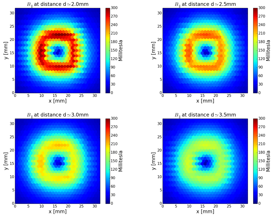
Figure A.8.: Horizontal magnetic field at various distances above the magnet 12.
