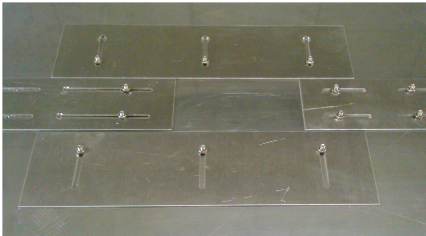
Figure 5.21.: The new rail for the glueing process. Again, the basis is an iron plate. The four aluminium plates with the long holes can be moved in one direction each. Once they are positioned correctly, they can be fixed via the screws and the nuts. In a first step the “upper” plate (related to the figure) and the one on the right side are fixed. After the stripes are put onto the iron plate and brought into line with the edges, the “lower” plate is moved towards them and then also fixed. This way, the stripes are bound in three directions. The plate on the left side can then be used to push them together and, after also being fixed, bound them in the remaining direction.
