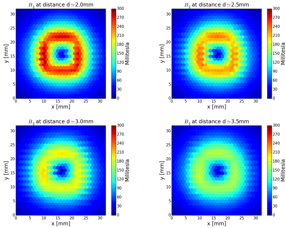
Figure A.15.: Horizontal magnetic field at various distances above the magnet 19.
